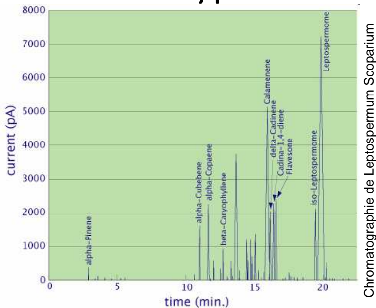
Chemical composition of pure East Cape manuka oil measured by gas chromatography and depicting many of the principal known peaks.
